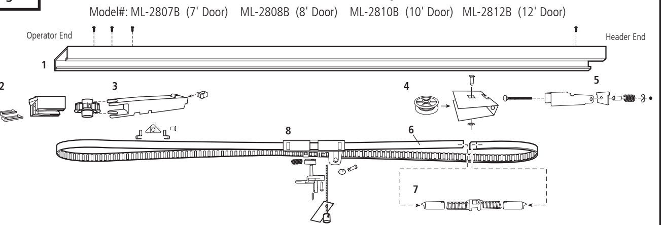
Belt Rail Assembly
