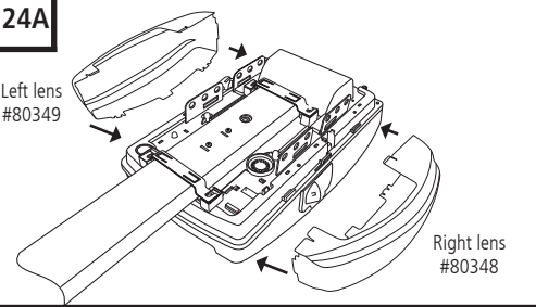
Hinge lamp lens downward line up tabs with slots in housing, and snap into place.
